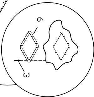
LIFT STRUT EXIT DOUBLER INSTALLATION
