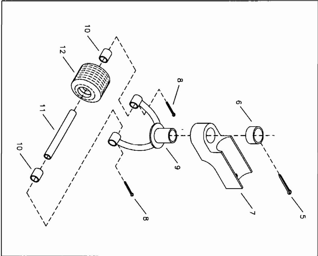
TAILWHEEL ASSEMBLY DETAIL
