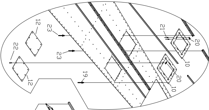
FWD TAILCONE ACCESS COVER ASSEMBLY
